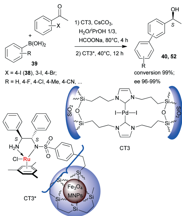
Scheme 16 Sequential SuC-ETH reactions catalysed by two heterogeneous catalysts containing anchored Pd and chiral Ru complexes. 134
