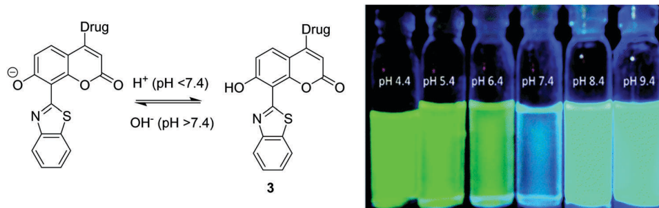
Fig. 3 A HBT-coumarin theranostic pH probe 3 for the monitoring of pH in cancer cells with UV activated drug release of chlorambucil. Measurement conditions: HEPES/ACN (7 : 3) buffer solution. Adapted with permission from ( J. Mater. Chem. B , 2015, 3 , 3490–3497). Copyright (2015) the Royal Society of Chemistry.
