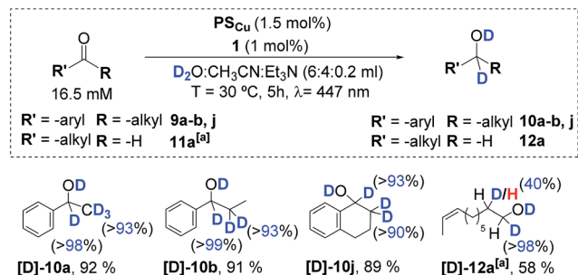
Scheme 5 Deuterium labelling studies of aromatic ketones ( 9a-b, j ), and aliphatic aldehydes ( 11a ). 1 (6 mol%), \text{PS}_{\text{Cu}} (6 mol%), substrate (4.4 mM) in \text{D}_2\text{O}:\text{CH}_3\text{CN}:\text{Pr}_2\text{EtN} (6:4:0.2 mL) irradiated (447 nm) for 24 h at -3^\circ\text{C} under \text{N}_2 . Isolated yields. Deuterium insertion analysed using NMR.
