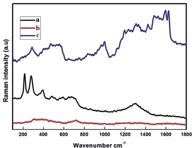
Fig. 3 Raman band of (a) Fe 3 O 4 (FMN); (b) β-CD-EDTA-Fe 3 O 4 (CEF); (c) β-CD-EDTA-Fe 3 O 4 /CPT (CEF-CPT).
