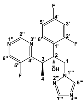
Fig. 1 The structure of voriconazole, \text{C}_{16}\text{H}_{14}\text{F}_3\text{N}_5\text{O} , molar mass of 349.12 \text{ g mol}^{-1} . ^1\text{H} , ^{13}\text{C} , and ^{19}\text{F} assignments are given below.
