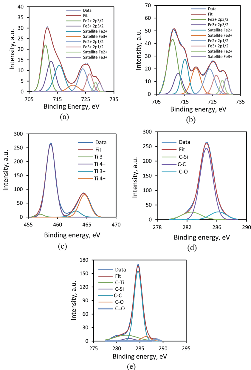
Fig. 3 XPS peak analysis of (a) Fe 2p peak on surface of \text{Fe}_3\text{O}_4 and (b) \text{Fe}_3\text{O}_4@\text{TiO}_2 , (c) Ti 2p peak on surface of \text{Fe}_3\text{O}_4@\text{TiO}_2 , and (d) C 1s peak on surface of \text{Fe}_3\text{O}_4 and (e) \text{Fe}_3\text{O}_4@\text{TiO}_2 .
