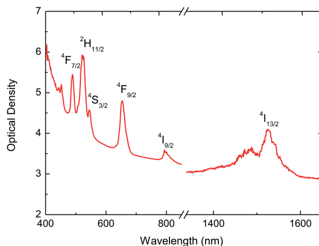
Fig. 5 Absorption spectrum for \text{BaTiO}_3:\text{Er}^{3+} 9\%-\text{Yb}^{3+} 1\% sample.
