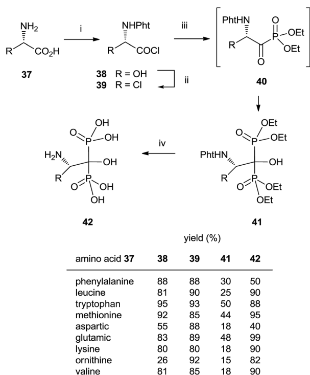
Scheme 11 Reagents and conditions: (i) N -(ethoxycarbonyl)phthalimide, NaHCO 3 , 0 °C, 5 min. (ii) SOCl 2 , CH 2 Cl 2 , 5 h, reflux. (iii) Triethyl phosphite, toluene, 1 h, 0 °C; then diethyl phosphite, Et 3 N, 1–3 h, 0–5 °C. (iv) 6 N HCl, reflux, overnight; then 5 N NaOH, pH = 4.4.
