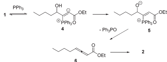
Scheme 2 Proposed mechanism.
