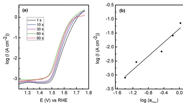
Fig. 7 (a) Tafel plots showing OER performance for Au/ \text{Co(OH)}_2 electrodeposited from 10 mM \text{Co(NO}_3)_2 \cdot 6\text{H}_2\text{O} at different deposition time, (b) effect of hydroxide ion activity on OER. The cyclic voltammetric experiments used to obtain the data was recorded at a sweep rate of 1 \text{mV s}^{-1} in 1 M NaOH.
