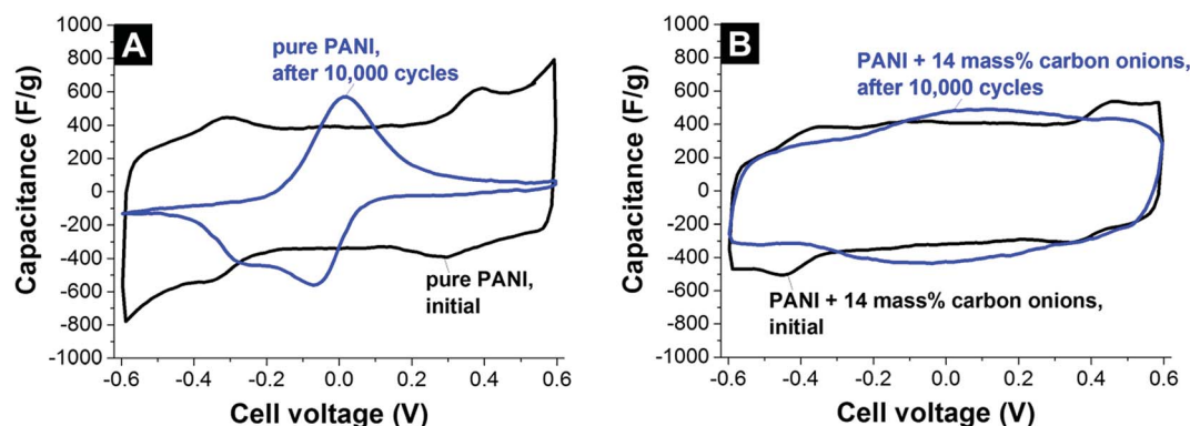
Fig. 15 Cyclic voltammograms of nanodiamond-derived carbon onions (1800 °C synthesis temperature) coated with PANI. Electrodes are PTFE-bound (3 mass%) and measured in a two-electrode configuration using 1 M H 2 SO 4 recorded at a scan rate of 1 mV s -1 . (A) Pure PANI electrodes. (B) Carbon onion/PANI composite with 14 mass% carbon onions. Data adapted from ref. 132.
