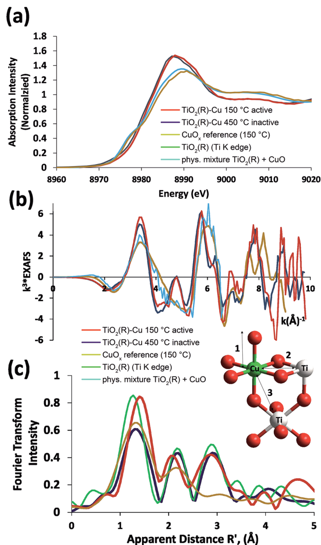
Fig. 4 XAS spectra of photocatalytically active \text{TiO}_2(\text{R}) -Cu (dried at 150^\circ\text{C} ) and inactive \text{TiO}_2(\text{R}) -Cu (calcined at 450^\circ\text{C} ) are compared to the reference data of \text{CuO}_x (prepared by heating), rutile \text{TiO}_2(\text{R}) (Ti K edge), and a physical mixture of \text{TiO}_2(\text{R}) and CuO. Data are presented as XANES (a), EXAFS (b) and Fourier transform of the EXAFS (c). The inset shows a structural model used for fitting.
