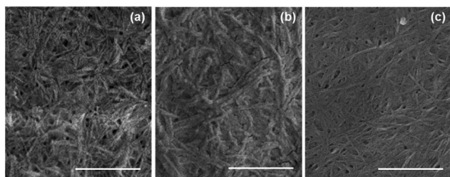
Fig. 5 SEM images of (a) xerogel-1,2, (b) xerogel-1 and (c) xerogel-2. Scale bars represent 500 nm.
