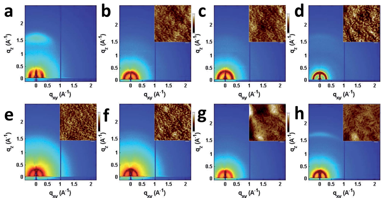
Fig. 5 GIWAXS images of pristine PBDTT-FITTE (a), PBDTT-FITTE:Ph1 (b), PBDTT-FITTE:Ph2a (c), PBDTT-FITTE:Ph2b (d), PBDTT-FITTE:T1 (e), PBDTT-FITTE:T2 (f), PBDTT-FITTE:TT1 (g), and PBDTT-FITTE:TT2 (h) films. AFM images of the blend films are shown in the insets and enlarged versions are available in Fig. S3.† All films were spin-coated on Si/SiO 2 from chloroform with 1 wt% DIO.
