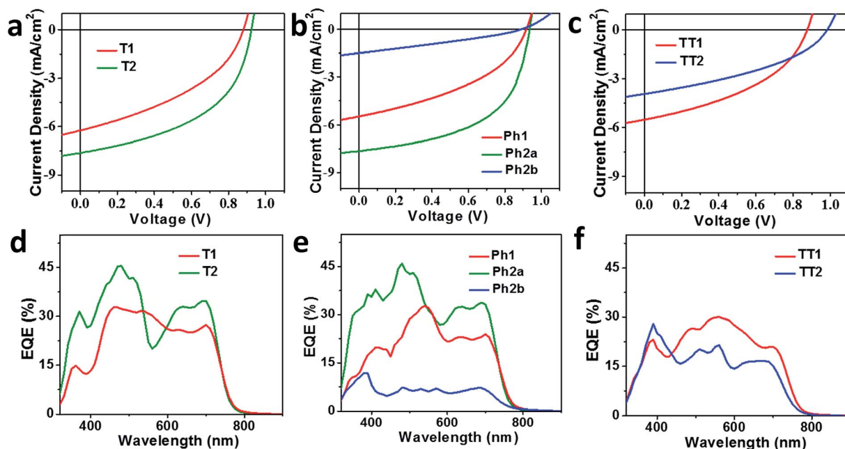
Fig. 4 J–V curves (a–c) and EQE spectra (d–f) of OPV devices based on T1 and T2 (a and d), Ph1, Ph2a, and Ph2b (b and e), and TT1 and TT2 (c and f) blended with the donor polymer PBDTT-FITTE.
