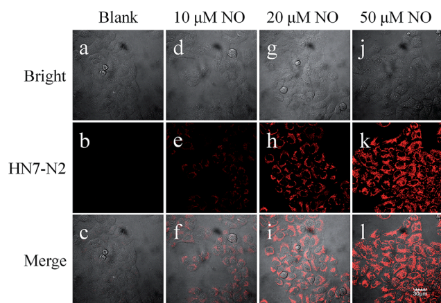
Fig. 9 Confocal fluorescence imaging of NO in HeLa cells with HN7-N2 (10 μM) for 30 min and then NO donor, diethylamine NONOate (from left to right: 0, 10, 20, 50 μM, respectively) for 30 min. Excitation at 543 nm for red emission of HN7-N2 (650–720 nm).
