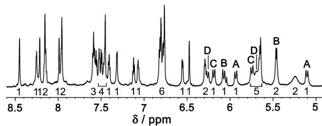
Fig. 8 ^1\text{H} NMR spectrum ( \text{CD}_3\text{NO}_2 , 800 MHz) of redissolved crystals of [\text{Ru}_4\text{Cd}_{12}(\text{L}^{\text{ph}})_{12}(\text{L}^{\text{naph}})_{12}](\text{PF}_6)_7(\text{BF}_4)_{25} . Integers under the signals are integral values (total 42). Labels (A–D) refer to the four pairs of doublets from diastereotopic methylene groups, identified from a COSY spectrum, which confirm the presence of two independent ligand environments with no internal symmetry and equal numbers of each type (see main text).
