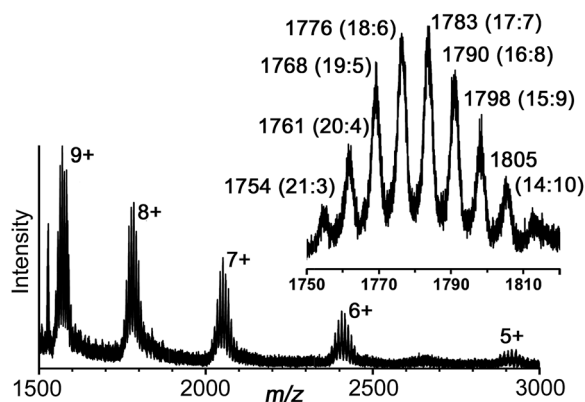
Fig. 9 Partial electrospray mass spectrum of redissolved crystals of [\text{Ru}_4\text{Cd}_{12}(\text{L}^{\text{ph}})_{12}(\text{L}^{\text{naph}})_{12}](\text{PF}_6)_7(\text{BF}_4)_{25} showing the sequence of signals associated with progressive loss of anions. For each charge, the presence of multiple closely-spaced signals is associated with different combinations of [\text{BF}_4]^- and [\text{PF}_6]^- anions. The inset shows the expansion of the set of signals around m/z 1780 for the 8+ ions: the number of [\text{BF}_4]^- and [\text{PF}_6]^- anions for each is shown in parentheses. Thus, the signal at m/z 1768 corresponds to \{[\text{Ru}_4\text{Cd}_{12}(\text{L}^{\text{ph}})_{12}(\text{L}^{\text{naph}})_{12}](\text{BF}_4)_{19}(\text{PF}_6)_5\}^{8+} , etc. For high-resolution expansions, see ESI.†
