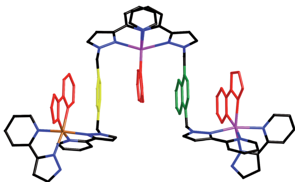
Fig. 7 Five-layer aromatic stack in the structure of [\text{Ru}_4\text{Cd}_{12}(\text{L}^{\text{ph}})_{12}(\text{L}^{\text{naph}})_{12}](\text{PF}_6)_7(\text{BF}_4)_{25} with electron-rich phenyl and naphthyl rings in yellow and green, respectively, and electron deficient pyrazolyl-pyridine units in red. Cd – purple; Ru – orange.
