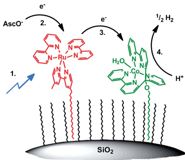
Scheme 4 Proposed reaction mechanism of photocatalytic H 2 production on hydrophobic silica: (1) photoexcitation of 1 to 1 *; (2) reductive quenching of 1 * to 1 - ; (3) electron transfer 1 - → 3 ; (4) H + reduction by 3 - .
