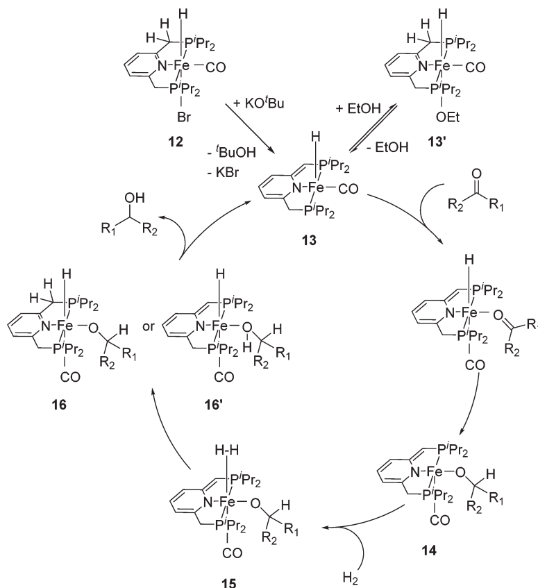
Fig. 7 Proposed catalytic cycle for the hydrogenation reactions of ketones using [(iPrPNCp)FeH(CO)Br] ( 12 ) as a pre-catalyst.
