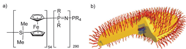
Fig. 14 Chemical structure of the block copolymer consisting of poly(ferrocenylsilane) and polyphosphazene ( R = \text{OCH}_2\text{CF}_3 ) blocks (a) and an idealized graphic representation of the pointed-oval-shaped micelles after crystallization-driven living self-assembly (b). Adapted with permission from A. Presa Soto et al. , Angew. Chem., Int. Ed. , 2010, 49 , 8220. Copyright 2010 Wiley-VCH. 33
