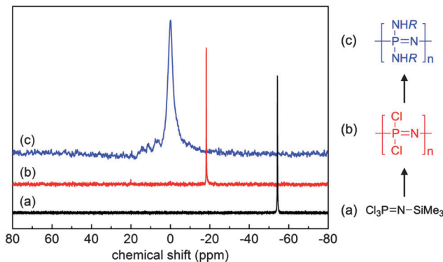
Fig. 4 Sample ^{31}\text{P}\{^1\text{H}\} NMR spectra of the monomer trichlorophosphoranimine \text{Cl}_3\text{P}(\text{N})\text{SiMe}_3 (a), polydichlorophosphazene [\text{N}(\text{P}(\text{Cl})_2)]_n (b) and a macrosubstituted poly(organo)phosphazene [\text{N}(\text{NHR})_2]_n (c) demonstrating the simple tracking of the reaction progression. Adapted from H. Henke et al. , J. Polym. Sci., Part A: Polym. Chem. , 2013, 51 , 4467. Copyright 2013 Wiley Periodicals, Inc. 12
