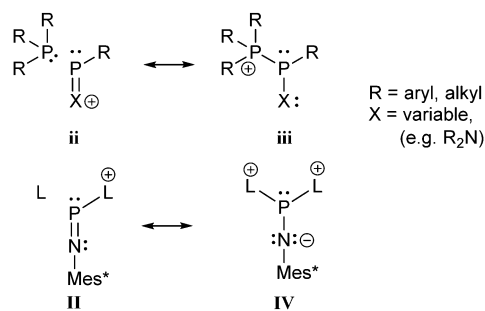
Scheme 26 Resonance structures describing a phosphane stabilized phosphonium ion (ii) and a phosphanylphosphonium ion (iii). Resonance structures II and IV from Scheme 20 are illustrated for reasons of comparison.
