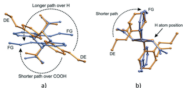
Fig. 18 Superimposition of the DE and FG molecules (by least-squares fit of respective C1, C11, C12 and C13 cyclobutane atoms) after 60 h of UV irradiation; (a) approximate top view of the cyclobutane ring showing the two possible paths taken by the phenyl-ethoxy group of the FG molecule undergoing a conformational change from the DE molecule; (b) side view of the cyclobutane ring giving an indication of the size of the carboxylic acid group.
