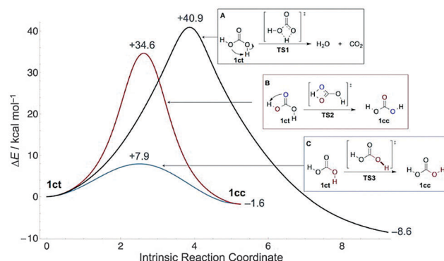
Fig. 1 Potential energy curves at CCSD(T)/CBS for disappearance of 1ct by decomposition into \text{H}_2\text{O} and \text{CO}_2 (A), [1,3]hydrogen transfer (B), or internal C–O bond rotation (C). The profiles are drawn in terms of computed arc length (in \text{u}^{1/2} bohr) along the intrinsic reaction path.
