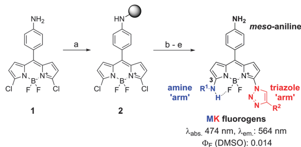
Scheme 1 Solid-phase synthesis of MK fluorogens. Reaction conditions: (a) CTC-PS, DIPEA, CH_2Cl_2 :DMF (1:1), r.t.; (b) NaN_3 , DMF, r.t.; (c) R^1NH_2 , DIPEA:DMF (1:4), r.t.; (d) R^2-C\equiv CH , CuI, L-ascorbic acid, r.t.; (e) TFA: CH_2Cl_2 (0.5:99.5), r.t.
