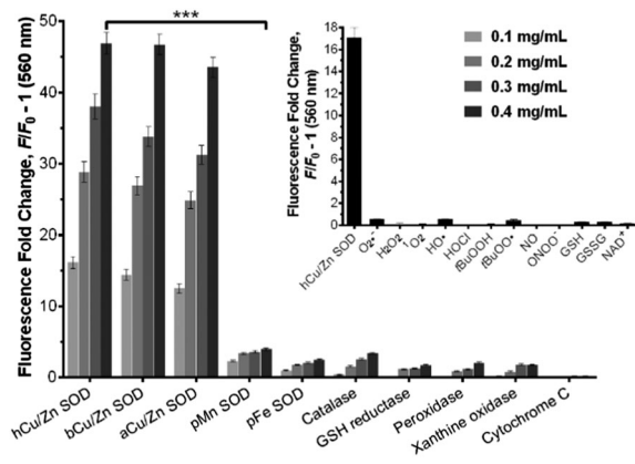
Fig. 2 Fluorogenic response of SODO upon binding to different proteins (at 0.1, 0.2, 0.3 and 0.4 mg mL^{-1} ) and metabolites (inset, ROS & RNS: 100 \mu M ) in 20 mM Tris-HCl buffer (pH = 7.4). \lambda_{exc} : 460 nm, \lambda_{em} : 560 nm. Values are represented as means and error bars as standard deviations ( n = 3 ), *** for p < 0.001 .
