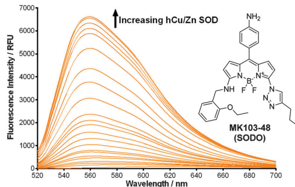
Fig. 1 Chemical structure and fluorescence spectra of SODO ( 10 \mu M ) after incubation with serial concentrations of hCu/Zn-SOD from 0.01 to 5 mg mL^{-1} in 20 mM Tris-HCl buffer (pH = 7.4). \lambda_{exc} : 460 nm. \Phi_F in hCu/Zn-SOD: 0.45.
