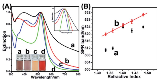
Fig. 5 The UV-vis spectra (A) of YS Au@AgPd NPs (a, black curve), OM-YS Au@AgPd NPs (b, red curve), CS Au@AgPd NPs (c, blue curve) and Au NPs (d, green curve). The curves are normalized with the intensity of the SPR maximum of the Au NPs. The Au NPs are 30 nm in size. The insets in the lower-left corner are the optical photos of the glass vials of the aqueous dispersions of the corresponding NPs (a–d). The inset in the upper-right corner highlights the variation of the SPR maximum of the Au cores in different NPs. The plots of the peak positions (B) of Au cores in the conventional YS Au@AgPd NPs (a, solid square) and OM-YS Au@AgPd NPs (b, solid circle) vs. the refractive index of different solvents.
