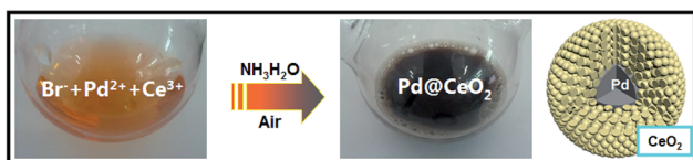
Scheme 1 The synthetic process of Pd@CeO 2 core@shell nanospheres.
