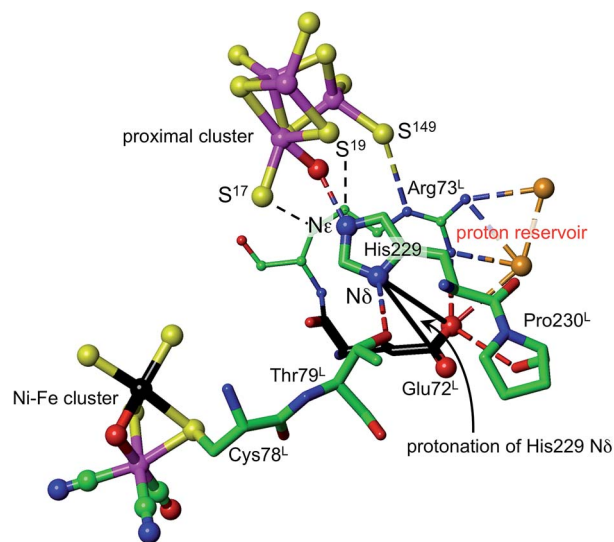
Fig. 5 The surroundings of His229 in PDB 4IUB (which contains OH on Fe1 of the proximal cluster, and bridging O in the Ni-Fe site, the Ni-B state). N \epsilon of His229 is hydrogen bonded to OH on Fe1, and is within hydrogen bonding distances of S 17 (3.3 Å) and S 19 (3.7 Å). N \delta of His229 is hydrogen bonded to the side-chain of Thr79 L , and is near (4.2 Å, black connectors) the carboxylate side-chain atoms (red spheres) of Glu72 L . These same carboxylate atoms are engaged in a hydrogen bonding network involving two water molecules (orange spheres), the side-chain NH 2 groups of Arg73 L , and carbonyl of Pro230 L . This is the proton reservoir domain. Additional hydrogen bonds between the proton reservoir and its surrounds are not shown.
