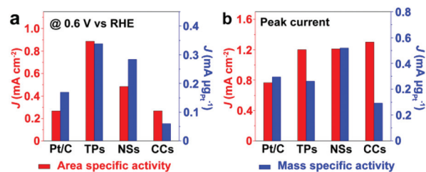
Fig. 6 Comparison of the area specific activity and mass specific activity of Pt/C and Pt/Ru NCs/C composites at 0.6 V vs. RHE and the peak in the forward scan of corresponding CV curves in Fig. 5a. TPs, NSs and CCs in this figure stand for Pt/Ru TPs/C, Pt/Ru NSs/C and Pt/Ru CCs/C, respectively.
