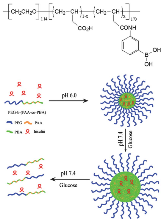
Fig. 11 Structure of PEG- b -(AA-co-AAPBA) and schematic illustration of the formation, swelling and dissociation of insulin-loaded micelles. (Reprinted with permission from ref. 18. Copyright © 2009, American Chemical Society.)
