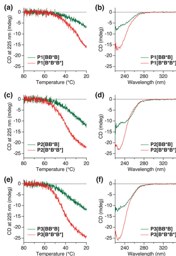
Fig. 3 CD cooling curves (a, c and e) and spectra at 20 °C (b, d and f) for Pn[BB*B] (green) and Pn[B*B*B*] (red) ( n = 1, 2, and 3; c BTA = 50 μM in DCE; cooling rate: 1 °C min −1 ). (a, b) P1 (c, d) P2 , and (e, f) P3 series of polymers.
