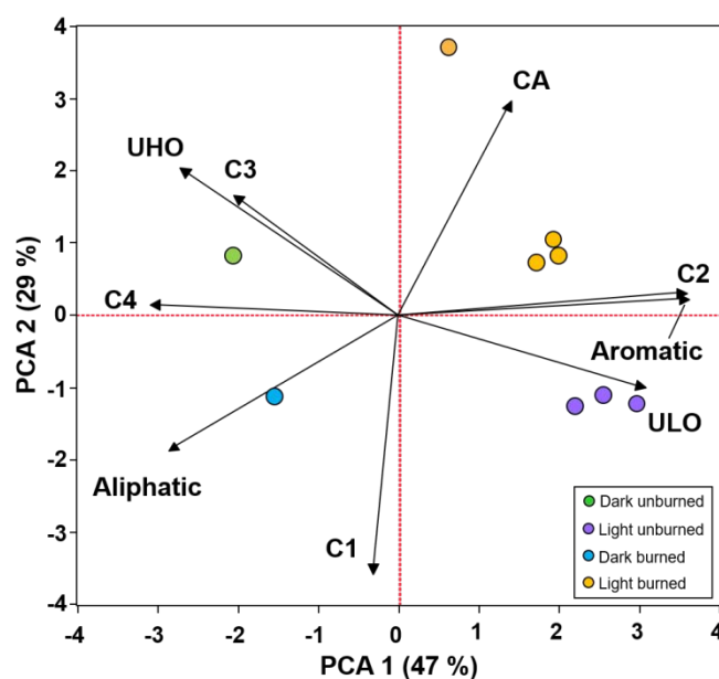
Figure 4: PCA analysis of loadings from PARAFAC (C1 – C4) and aliphatic, unsaturated low oxygen (ULO), unsaturated high oxygen (UHO), aromatic and condensed aromatic (CA) of data derived from FT-ICR MS for dark unburned (green), light unburned (purple), dark burned (blue) and light burned (gold).
