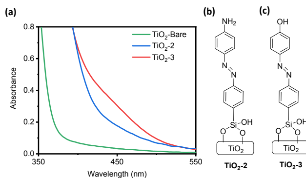
Fig. 3. (a) UV-Vis spectra comparing the solid-state absorption spectra of TiO 2 -Bare , TiO 2 -2 and TiO 2 -3 . Structures of (b) TiO 2 -2 and (c) TiO 2 -3 .
