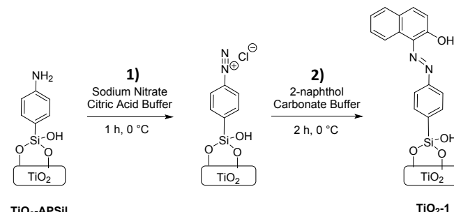
Scheme 2. Diazo coupling reaction to form TiO 2 -1 including 1) diazotization and 2) 2-naphthol coupling steps.
