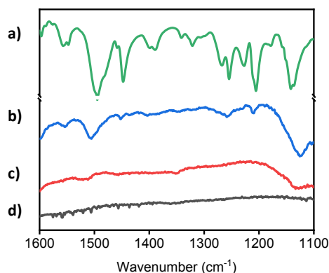
Fig. 2. ATR-FTIR spectra of a) Sudan I, b) TiO 2 -1 , c) TiO 2 -APSil , and d) TiO 2 -Bare . Spectra b through d were rescaled, to the same degree, in order to more easily compare their features with the powder sample, a.
