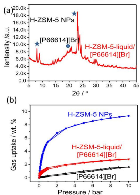
Fig. 3 a) XRD Pattern of H-ZSM-5-liquid/[P66614][Br] (Star: H-ZSM-5 NPs, Circle: [P66614][Br]); b) CO 2 adsorption-desorption isotherms of H-ZSM-5 NPs, [P66614][Br] and H-ZSM-5-liquid/[P66614][Br] collected at 298 K, respectively.
