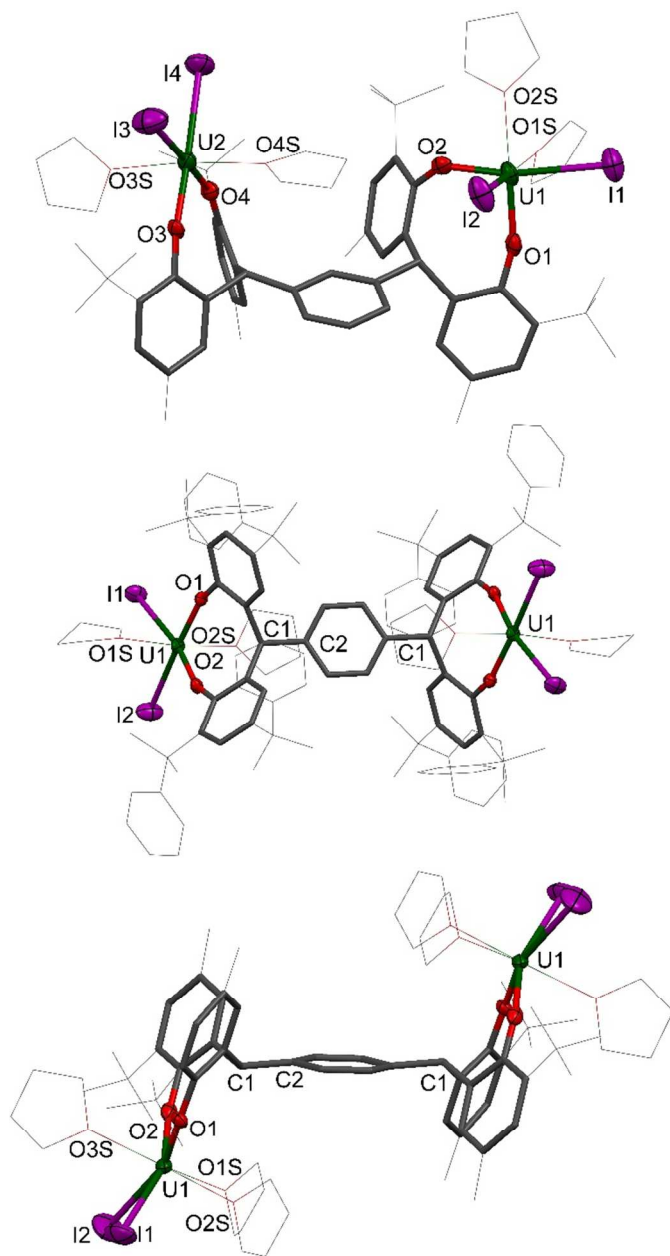
Figure 1 Solid-state structures of 1^P (upper, side view), 1^{P*} (middle, top view) and 1^M (lower, side view). For clarity, hydrogen atoms and lattice solvent molecules are omitted (displacement ellipsoids are drawn at 50 % probability, the remaining atoms and bonds shown as capped stick or wireframe). Selected bond lengths (Å) and angles (°) for 1^P : U1-O1 2.108(5), U1-O2 2.117(5), U1-I1 3.0970(8), U1-I2 3.1094(8), U1-O1-C11 157.4(4), U1-O1-C21 156.8(4). For 1^{P*} : U1-O1 2.105(4), U1-O2 2.106(4), U1-I1 3.0553(4), U1-I2 3.0472(5), U1-O1-C11 152.9(3), U1-O1-C21 159.1(3). For 1^M : U1-O1 2.132(12), U1-O2 2.080(11), U2-O3 2.110(9), U2-O4 2.129(10), U1-I1 3.0643(16), U1-I2 2.9860(14), U2-I3 3.0109(18), U2-I4 3.0562(14), U1-O1-C11 138.7(9), U1-O1-C21 161.1(10), U2-O3-C31 154.1(9), U2-O4-C41 156.0(9).
