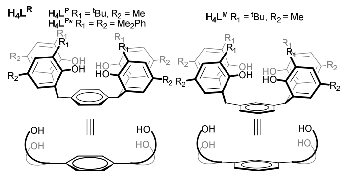
Figure 1 The substituted tetraphenols H 4 L R (with both para and meta substituted arene cores) and the new aryl-substituted H 4 L P* .
