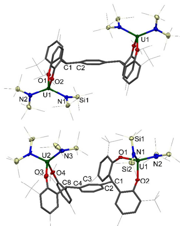
Figure 2 Solid-state structures of 2^P (upper, side view), and 2^M (lower, side view). For clarity, all methyl groups, hydrogen atoms, and lattice solvent molecules are omitted (displacement ellipsoids are drawn at 50 % probability, the remaining atoms and bonds shown as capped stick). For 2^{P*} see SI. Selected bond lengths (Å) and angles (°) for 2^P : U1-O1 2.1033(13), U1-O2 2.1362(13), U1-N1 2.2580(16), U1-N2 2.2479(17), U1-O1-C11 152.17(12), U1-O2-C21 146.77(12); 2^M : U1-O1 2.130(4), U1-O2 2.110(4), U2-O3 2.138(5), U2-O4 2.112(4), U1-N1 2.265(5), U1-N2 2.254(6), U2-N3 2.228(5), U2-N4 2.264(6), U1-O1-C11 141.5(4), U1-O2-C21 157.1(4) U2-O3-C31 138.5(4), U2-O4-C41 157.4(4).
