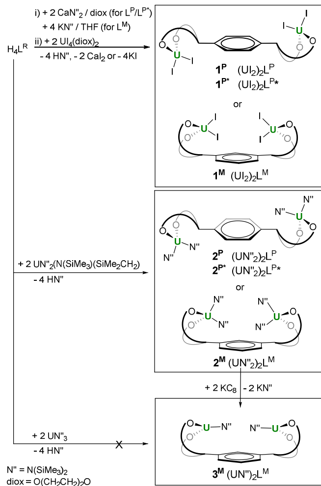
Scheme 1 Syntheses of (U^{IV})_2 and (U^{III})_2 complexes of bridged tetra-aryloxo ligands L^P , L^{P^*} and L^M .
