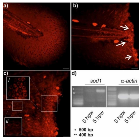
Fig. 3 In vivo imaging of Cu/Zn SOD in inflamed zebrafish after treatment with SODO (10 \mu M). a) Unwounded tail fin of a zebrafish embryo (3 dpf). b) Tail fin of a zebrafish embryo (3 dpf) 5 h after wounding (5 hpw). Strong fluorescence emission is observed towards the wound margin (white arrows). Bright spots in a) and b) away from the wound edge correspond to auto-fluorescence signals from pigment cells. c) High magnification images showing bright fluorescence from SODO at the wound margin (i) compared to non-fluorescent unwounded areas (ii). d) Semi-quantitative RT-PCR of sod1 and \alpha -actin genes at 0 and 5 hpw with corresponding ladders. Scale bars (a, b): 40 \mu m; (c): 20 \mu m.
