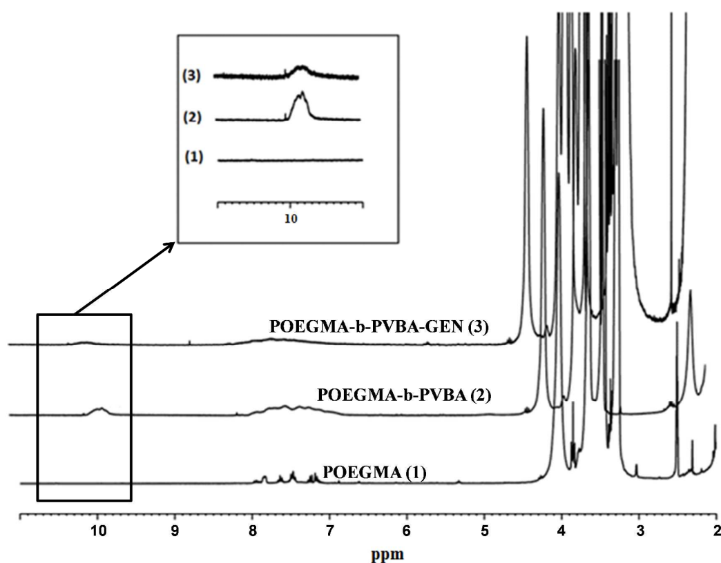
Figure 2. ^1\text{H} NMR spectra of purified POEGMA- b -PVBA-GEN overlaid with POEGMA- b -PVBA and POEGMA.
