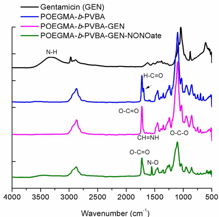
Figure 3. ATR-FTIR spectra of POEGMA- b -PVBA-GEN-NONOate compared with POEGMA- b -PVBA-GEN, POEGMA- b -PVBA and gentamicin.
