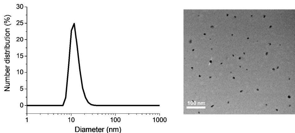
Figure 1. Dynamic light scattering (DLS) graph (left) and TEM image (right) depicting the size of POEGMA- b -PVBA-GEN nanoparticles.
