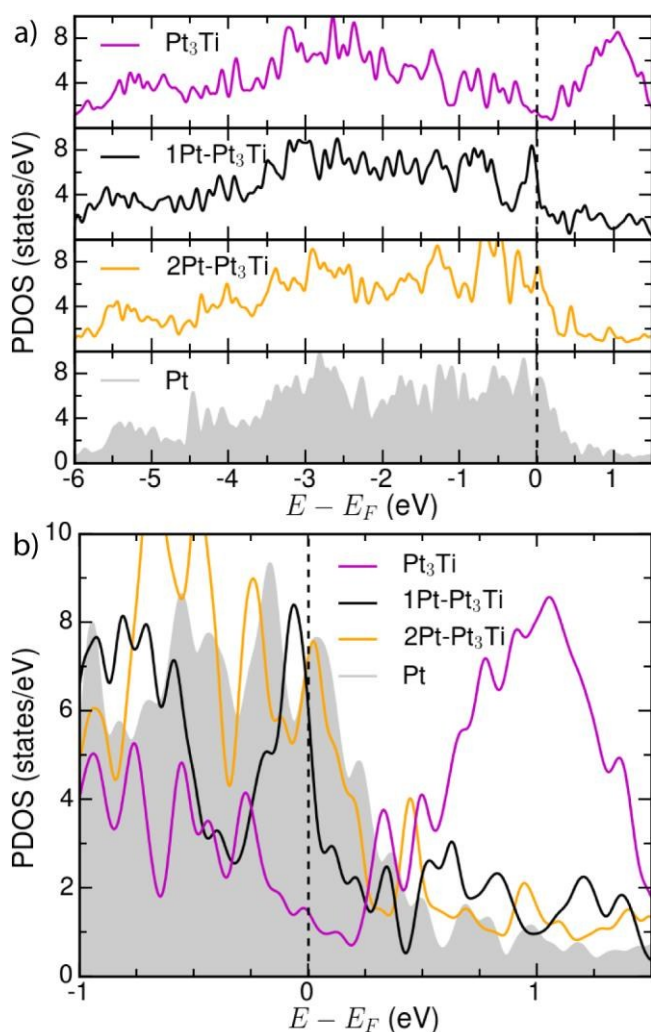
Fig. 4 (a) Total d-PDOS used to calculate the d-band centers ( \epsilon_d ) for \text{Pt}_3\text{Ti} , \text{Pt-Pt}_3\text{Ti} , 2\text{Pt-Pt}_3\text{Ti} and \text{Pt}(111) -substrates (see Table 1). (b) Comparison of the total d-PDOS of the simulated terminations in the energy range around E_F .
