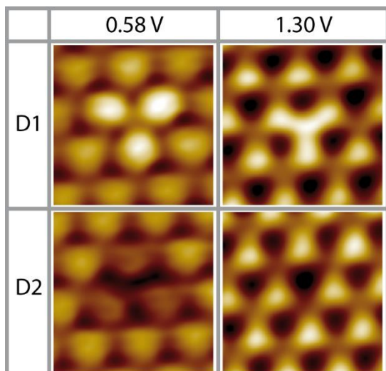
Fig. 5 Two different characteristic surface defects on S1 (Pt-Pt 3 Ti), D1 and D2 (0.58 V, 0.48 nA; 1.30 V, 0.11 nA; low pass filtered; 1.7 nm x 1.7 nm).
