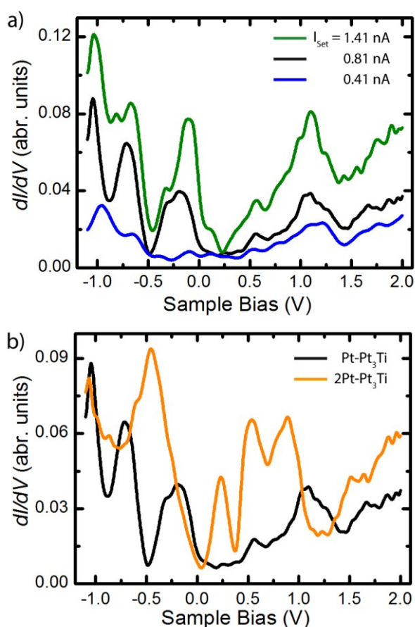
Fig. 3 (a) UHV-STS recorded on the Pt-Pt 3 Ti termination at different heights above the crystal defined by the STS set-point parameters: V_{set} = -1.10 V, I_{set} = 0.41 nA, averaged over 10 single curves (blue), V_{set} = -1.10 V, I_{set} = 0.81 nA, averaged over 4 single curves (black), V_{set} = -1.10 V, I_{set} = 1.41 nA, averaged over 20 single curves (green). (b) Comparison of UHV-STS curves taken from Pt-Pt 3 Ti ( V_{set} = -1.10 V, I_{set} = 0.81 nA, averaged over 4 single curves (black)) and 2Pt-Pt 3 Ti ( V_{set} = -
