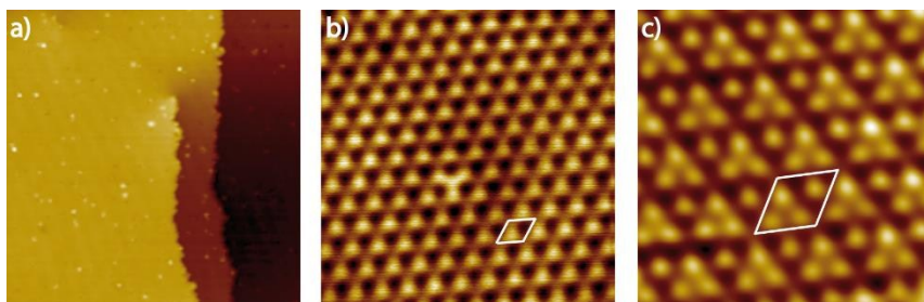
Fig. 1 (a) UHV-STM image of the Pt 3 Ti surface with one atomic step and a screw dislocation (sample 1 = S1). Furthermore, some surface defects and adsorbates are visible (57.5 nm x 57.5 nm, 2.31 V; 0.01 nA). (b) High-resolution image with one surface defect. The Ti induced p(2x2) superstructure is clearly visible (S1, 6.25 nm x 6.25 nm, 1.3 V, 0.11 nA); (c) UHV-STM of the Pt 3 Ti surface after repeated cleaning cycles with atomic resolution (S2, 2.50 nm x 2.50 nm, 0.006 V, 7.9 nA, (low pass filtered)).
