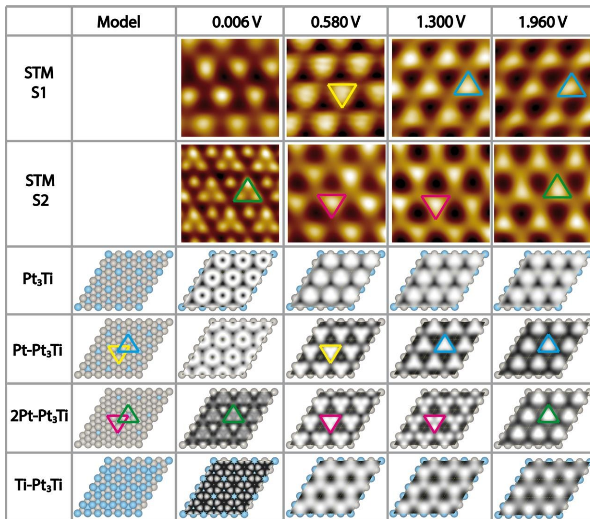
Fig. 2 Comparison of high-resolution UHV-STM images (1.5 nm x 1.5 nm, low pass filtered) and ab-initio DFT calculations of the \text{Pt}_3\text{Ti}(111) surface. In the first and second row STM images of sample 1 (S1) and sample 2 (S2), prepared under different conditions (see text), are shown for selected sample bias voltages, indicated at the top of each column. The calculated STM images corresponding to the respective bias voltages for four different surface terminations, i.e. bulk termination, Pt layer termination, two layers of Pt termination and Ti layer termination, are shown in row 3 to row 6. For the explanation of the colored triangles see text.
