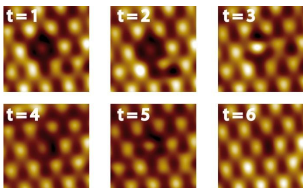
Fig. 6 High-resolution UHV-STM images of Pt-Pt 3 Ti (2.1 nm x 2.1 nm) showing the healing process of a defect by restructuring (T = 77 K). Time difference between two following STM images: \Delta t = 170 s (0.94 V; 0.08 nA, low pass filtered).
