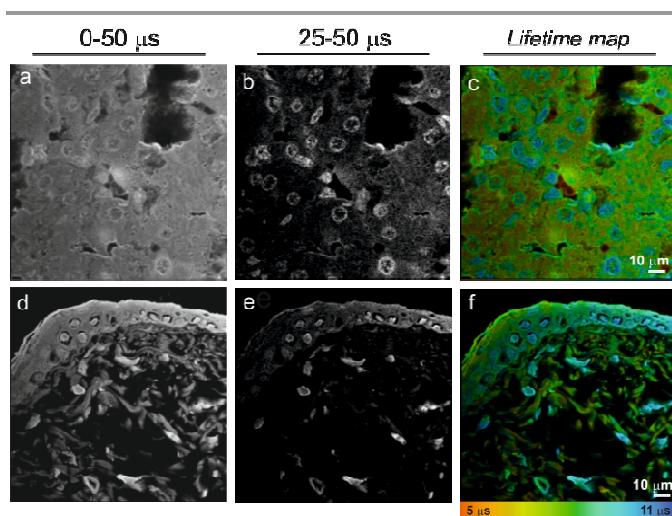
Figure 4: Time gated images of liver (a-c) and skin (d-f) 10 \mu\text{m} tissue sections, showing how the PLIM method in conjunction with the Pt(II)-based imaging agent 1 can be used to remove autofluorescence, improving image contrast – cell nuclei clearly much more visible in the time-gated image at later times. a, b, d, e – intensity images, c and f – lifetime maps.
