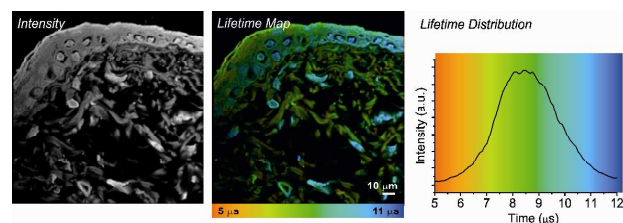
Figure 3: TP-PLIM imaging of histological section (10 \mu\text{m} ) of rat skin stained with 1 showing a stratified epithelial upper layer (the epidermis, containing keratinocytes) and dermis (containing fibroblast cells and collagen fibres).
