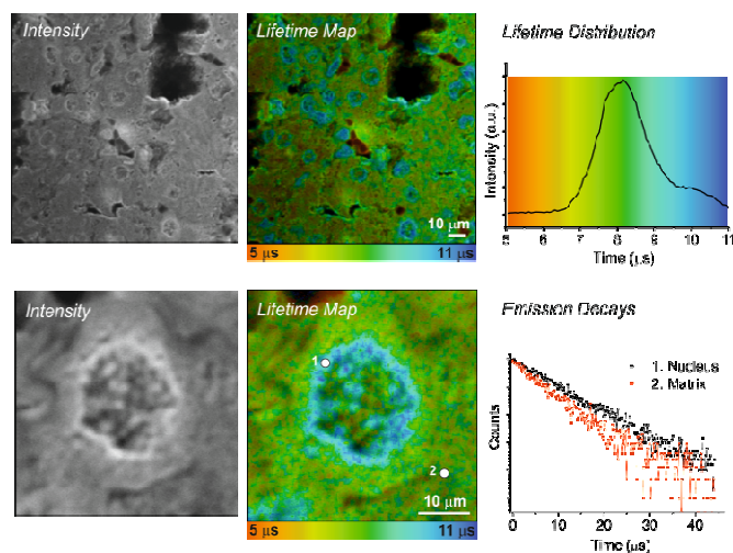
Figure 2: TP-PLIM imaging of fixed rat liver tissue section stained with 1 . Bottom: TP-PLIM imaging at higher magnification focusing on just a single nucleus within the tissue. Tissue section thickness 10 \mu\text{m} ; scale-bar - 10 \mu\text{m} .
