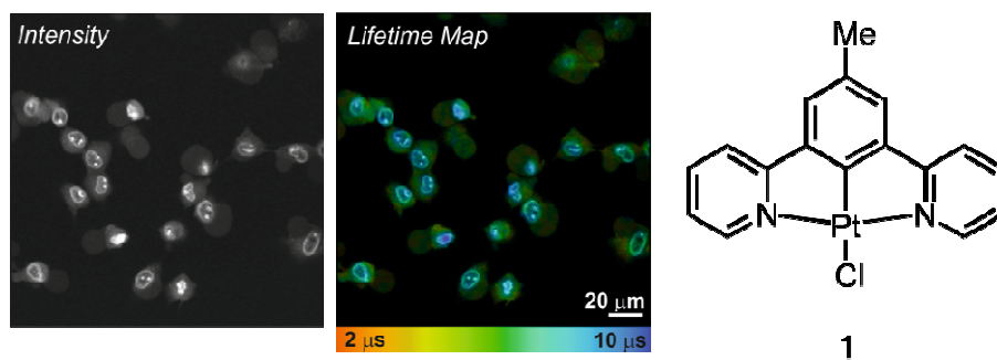
Figure 1: TP-PLIM imaging of live RN22 Schwannoma cells stained with complex 1 (50 μm, 5 min at 37°C). The chemical structure of 1 is shown on the right
