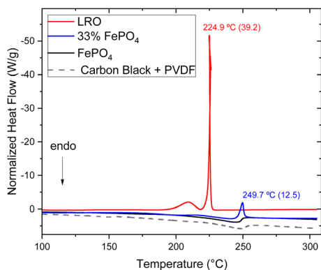
Fig. 4 DSC curves of pure LRO (red line), pure \text{FePO}_4 (black line) and a LRO: \text{FePO}_4 blend containing 33% \text{FePO}_4 (blue line). A control experiment is also included (dashed black line) with electrodes containing no active material and only the PVDF binder and carbon black. Heating rate was 10\text{ °C min}^{-1} .
