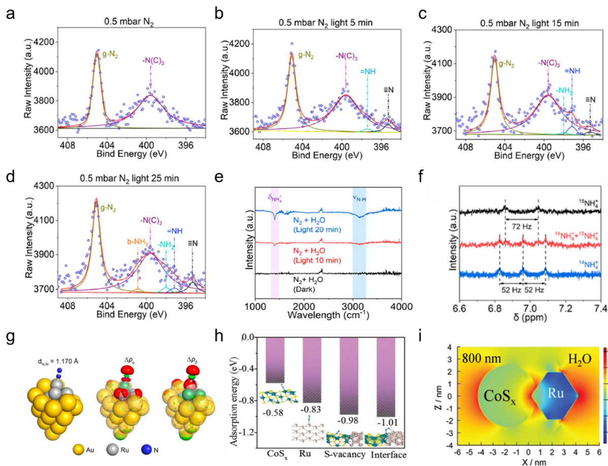
Fig. 12 (a)–(d) N 1s XPS spectra of \text{AuRu}_{0.31} . (e) In situ DRIFTS spectra recorded for \text{N}_2 + \text{H}_2\text{O} over \text{AuRu}_{0.31} under irradiation conditions. (f) ^{15}\text{N} NMR spectra of solution after the \text{N}_2 fixation reaction in the ^{15}\text{N}_2 , ^{15}\text{N}_2 + ^{14}\text{N}_2 , or ^{14}\text{N}_2 atmosphere. (g) Optimized structures of \text{N}_2 adsorbed on the AuRu cluster. Reproduced with permission. 82 Copyright 2019, American Chemical Society. (h) Adsorption energies of \text{N}_2 on different sites. FDTD electric field distribution. (i) FDTD electric field distribution at Ru/ \text{CoS}_x nanoparticle (800 nm irradiation) observed from \gamma -axis (vertical to incident light). Reproduced with permission. 83 Copyright 2019, Wiley-VCH.
