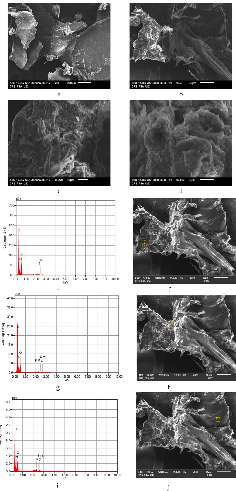
Fig. 2 SEM images of SE-CP at different magnifications: (a) 200 µm, (b) 50 µm, (c) 10 µm and (d) 5 µm and EDX spectra of the SE-CP biomaterial from an acid-etched section (e), (g) and (i) and corresponding SEM images (f), (h) and (j).
