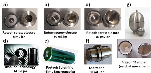
Fig. 3 Commercially available jars used for vibrational ball milling. The internal shape of the top and bottom caps are hemispheres, connected through a cylindrical section. (a)–(f) Used under horizontal vibratory motion using ball mills depicted in Fig. 2(b). The milling jar in (g) is used for vertical motion using ball mills depicted in Fig. 2(c).
