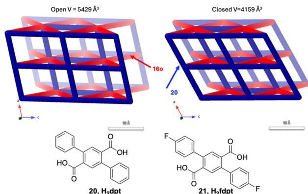
Fig. 13 [\text{Cd}(16\text{o})(\text{dpt})_2] LMA-1- \alpha and [\text{Cd}(16\text{c})(\text{dpt})_2] LMA-1- \gamma 1-UV both described by the 8-connected hex-net. LMA-1- \alpha can go through two subsequent phase transitions reducing the cell volume to form LMA-1- \beta and then LMA-1- \gamma 1 which are all colourless. Then LMA-1- \gamma 1 can go through a SCSC photoconversion to finally give the dark blue LMA-1- \gamma 1-UV. 84 The DAE based network links (red) shrink from 20.2 Å to 18.1 Å going from the open to the closed form.
