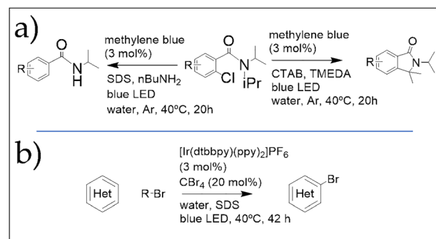
Fig. 11 (a) Reaction scheme of the micellar photocatalyzed activation of carbon-halide bonds, enabling controllable mechanistic switch between aromatic alkylation and dealkylative hydrogenation. (b) Reaction scheme of the Minisci-like halogenation of inactivated heteroarenes, enabled by photo-micellar catalysis. Both works were reported by Giedyk et al. 78,79
