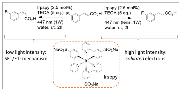
Scheme 2 Reaction scheme of the light intensity dependent reaction modality allowed by the use of the photocatalyst Irppy in water. Namely, the trans – cis isomerization (left, one-photon mechanism) and hydrogenation (right, two-photon pathway) with the substrates trans -3-fluorocinnamic acid using the blue-light driven photocatalytic system in water. 65
