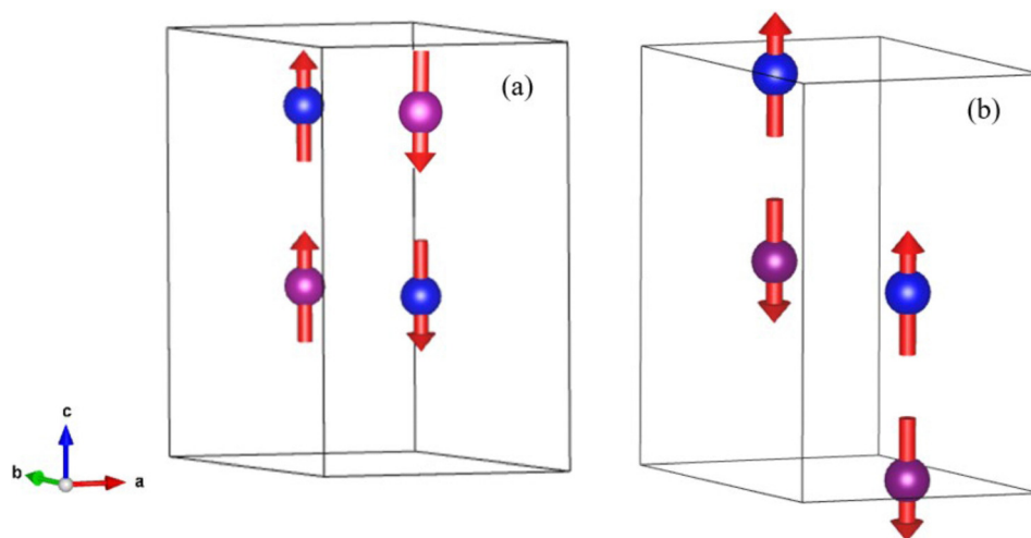
Fig. 7 Magnetic spin structure (red arrows) determined for (a) \text{MnCoMo}_3\text{O}_8 and (b) \text{MnFeMo}_3\text{O}_8 within the unit cell (black outline) at 2 K from the Rietveld refinement of powder neutron diffraction data. The blue and pink spheres represent manganese on the Mn1 (tetrahedral) and Mn2 (octahedral) crystallographic sites respectively.
