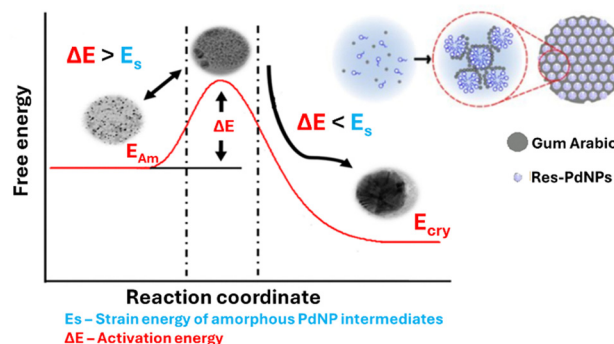
Fig. 3 Crystal growth of palladium nanoparticles influenced by GA, and a schematic illustration of the crystallization mechanism of amorphous palladium nanoparticles.
