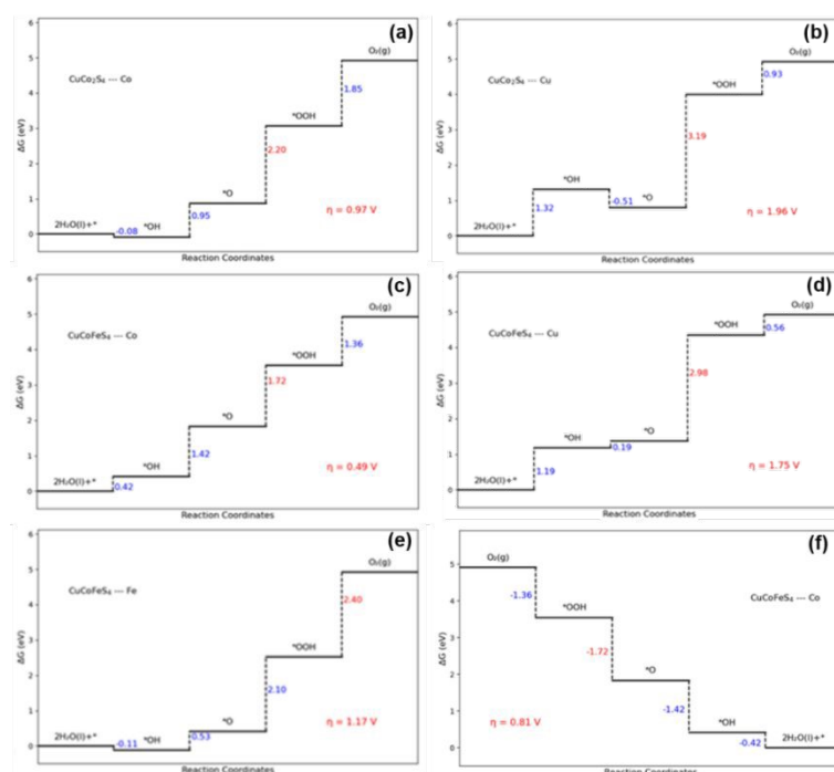
Figure 12: Free energy profile on (a) Co (b) Cu active sites in \text{CuCo}_2\text{S}_4 for OER mechanism Free energy profile in \text{CuCoFeS}_4 for OER mechanism on (c) Co (d) Cu and (e) Fe active sites (f) Free energy profile on Co active site in \text{CuCoFeS}_4 for ORR mechanism
