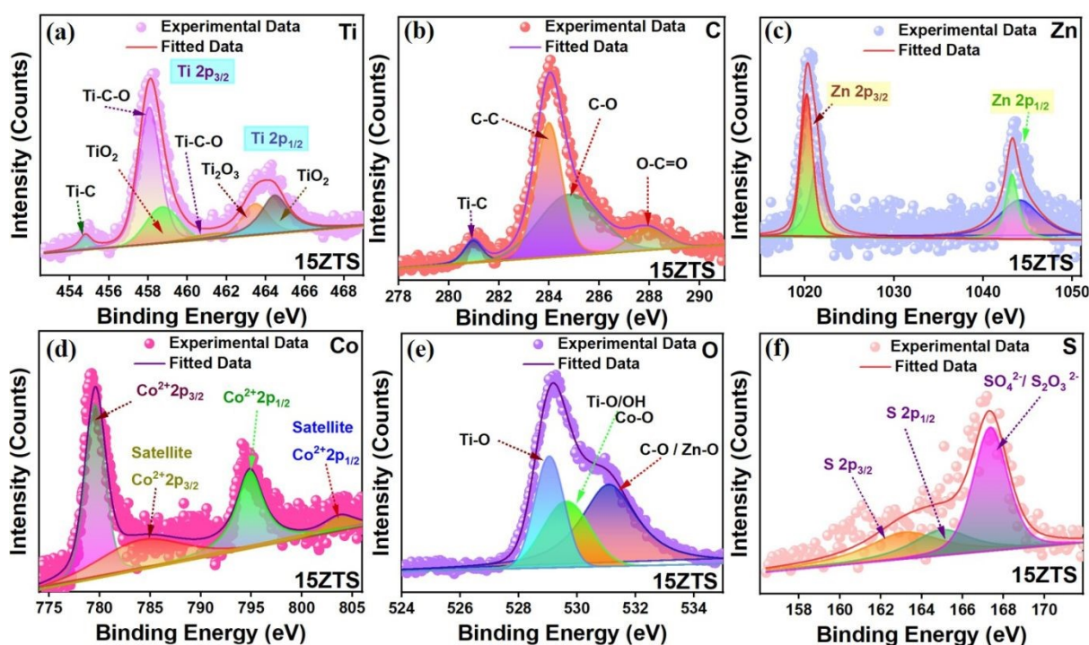
Fig. 2 High resolution XPS spectra for (a) Ti, (b) C, (c) Zn, (d) Co, (e) O and (f) S in 15ZTS.
