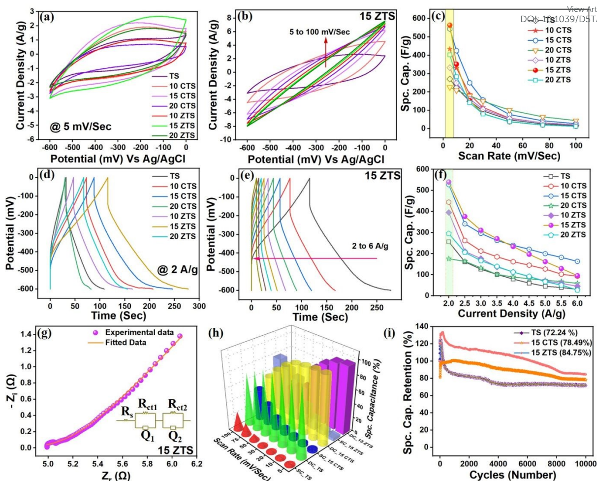
Fig.3 (a) CV curves of individual compositions at 5 mV/Sec, (b) voltammograms of 15ZTS at various scan rates (5 to 100 mV/Sec), (c) retention performance of all compositions across scan rates, (d) GCD curve at a current density of 2 A/g for all compositions, (e) GCD curves of 15ZTS at various current densities (2 to 6 A/g), (f) retention capability of TS and 10,15,20Z/CTS at various current densities, (g) EIS curves of 15ZTS, (h) comparative plot of calculated surface and diffusion-controlled capacitance (by Dunn's method) of TS and 15Z/CTS, and (i) specific capacitance retention of TS, 15Z/CTS after 10,000 CV cycles.
