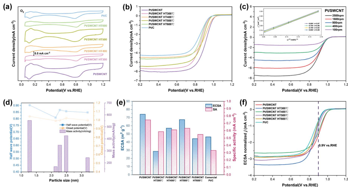
Fig. 6 Electrochemical performance of the Pt/SWCNT catalysts in 0.1 M \text{HClO}_4 solution: (a) cyclic voltammetry curves in \text{O}_2 -saturated solution, (b) linear sweep voltammetry curves in \text{O}_2 -saturated solution at 1600 rpm, (c) RDE polarization profiles of Pt/SWCNT at various rotation speeds and the respective Koutecky–Levich plots for different voltages, and (d) mass activity ( \text{mA mg}^{-1}\text{-Pt} ) comparison as a function of the Pt nanoparticle size, (e) summary of ECSA and SA values for all catalysts, and (f) ECSA-normalized LSV curves.
