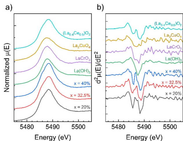
Fig. 2 \text{La } L_3 absorption edge (a) and second derivative (b) in \text{Ce}_x(\text{SmPrLaY})_{1-x}\text{O}_{2-\delta} and measured standards.
