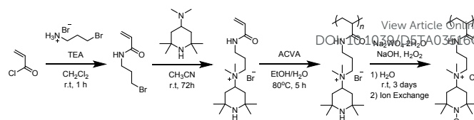
Scheme 1 Synthetic route to the TEMPO-substituted polyelectrolyte ( P1 ).
