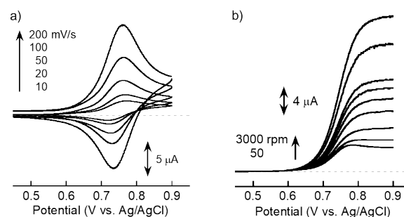
Fig. 3 Voltammetric responses obtained for 2 mM P1 dissolved in the aqueous electrolyte. (a) Cyclic voltammetry scanned at 10, 20, 50, 100, and 200 mV/s. (b) Hydrodynamic voltammograms. The electrode disk was rotated at 50, 100, 200, 400, 600, 1000, 2000, and 3000 rpm.
