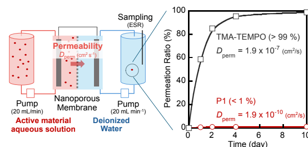
Fig. 4 Configuration of the cell for permeation test and related experimental result. The active materials kept flowed at 20 mL min -1 to proceed with permeation to the other cell with only water.
