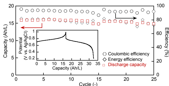
Fig. 5 Cycle performance of the prototype RFB with 0.25C, 20 Ah/L (0.75 M). Inset: Charge-discharge curves of the 1 st cycle.
